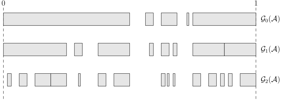
Figure 1. The collections \mathcal{G}_n(\mathcal{A}) .
