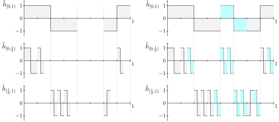
Figure 2. The first three functions of a (\chi_I)_{I \in \mathcal{D}} -faithful Haar system (\tilde{h}_I)_{I \in \mathcal{D}} which is extended to a faithful Haar system (\hat{h}_I)_{I \in \mathcal{D}} by adding the dashed Haar functions with the light blue shading.
